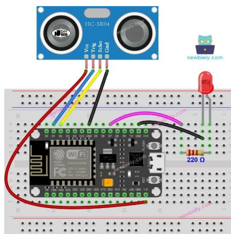
Figura 5 – LED. Fonte: NewBiely.
